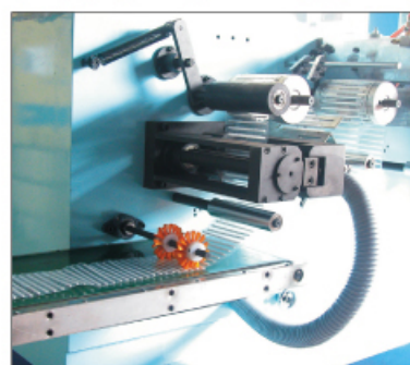
Conveyor for manual collection (Matches with vertical perforation)
